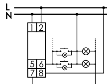
3 wires connection
