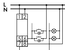
4 wires connection
